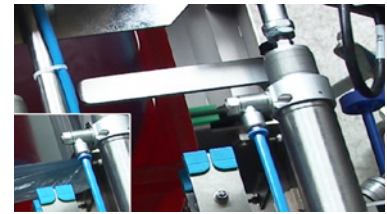
Mechanical grippers & spoons with bag detection
