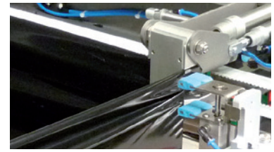
Mechanical grippers & spoon technology
