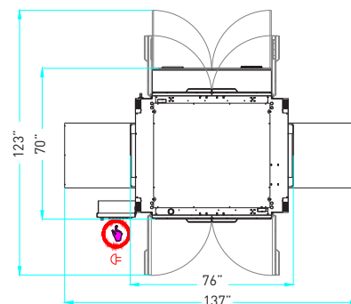
Machine height 86"
