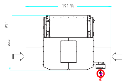
Machine height 192"
