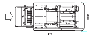
ODYSSEY-11-R Machine height 2350 mm
