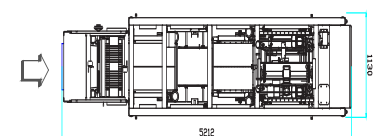
ODYSSEY-11-RS Machine height 2350 mm
