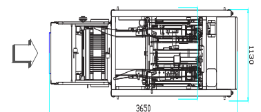
ODYSSEY-11-E Machine height 2350 mm
