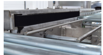
Box positioning by vertical side belts
