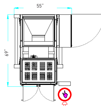
Machine height 94"
