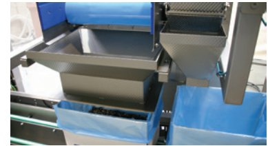
Gross weighing directly in the box
