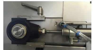
Demountable belt with quick release
