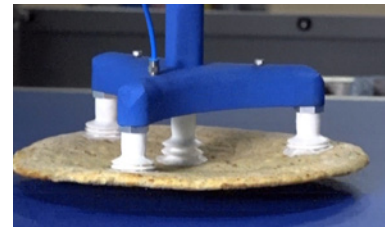
Delta robot
