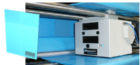
Optionaler Thermo-Transfer-Drucker
