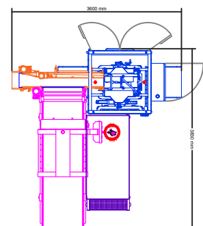
Machine height 3480 mm
