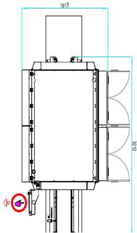
Machine height with film roll door closed: 83" Machine height with film roll door open: 89"
