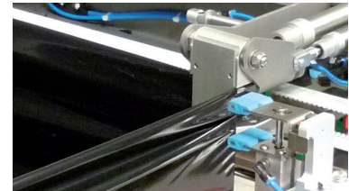
Mechanical grippers & spoon technology
