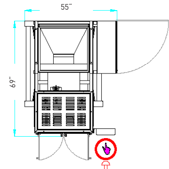
Machine height 94"
