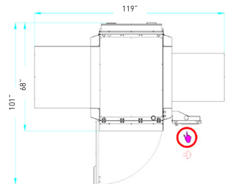
Machine height with film roll door closed: 82" Machine height with film roll door open: 89"
