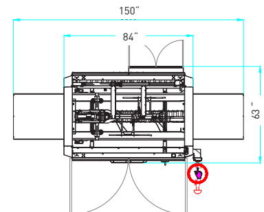
Machine height: 82"
