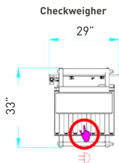
Checkweigher
