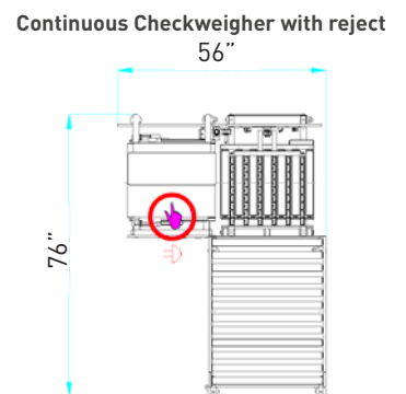
Continuous Checkweigher with reject
