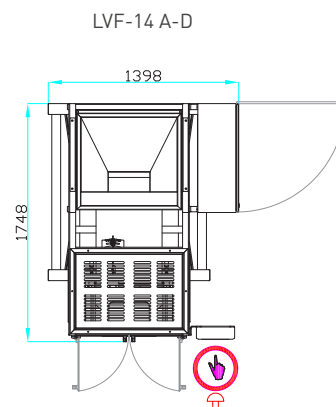
Machine height 2379 mm
