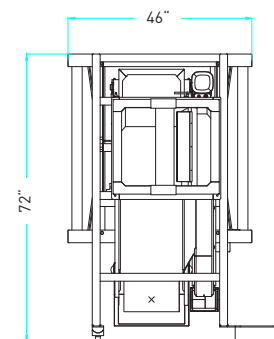
Sprocket driven homogeneous belt
