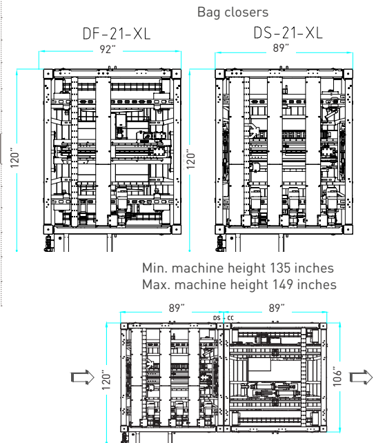
Combined bag closer with case closing module (optional)
