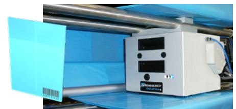
Optionaler Thermo-Transfer-Drucker
