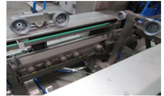
Box is clamped at three sides
