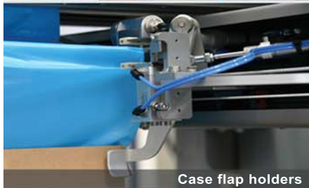
Mechanical grippers & spoons with air nozzle
