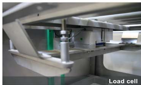
Load cell
